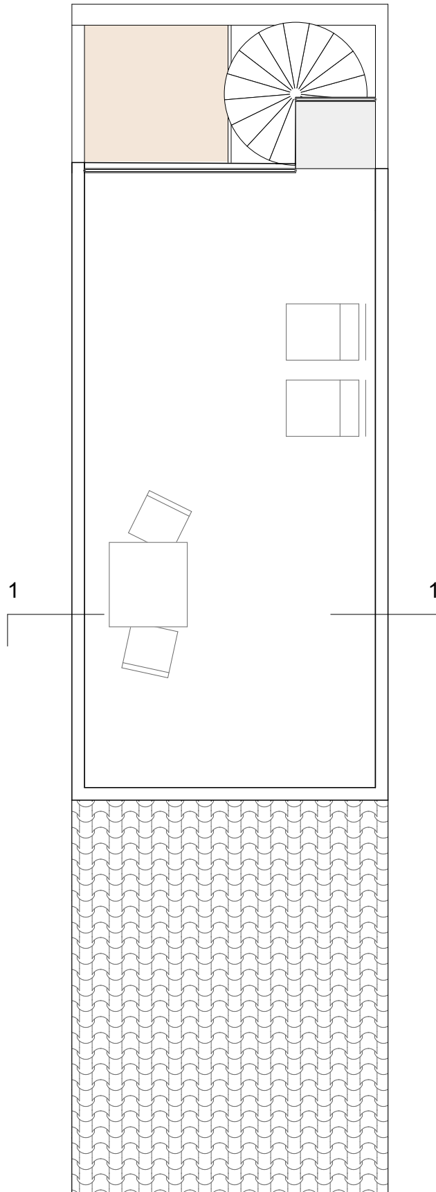
2dn Floor - Terrace scale 1/50
